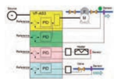
Example of 4 PID applications
