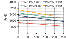
Clamping force diagram – interior gripping
