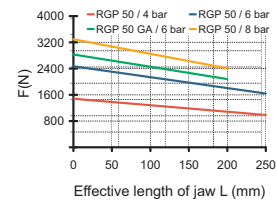
Clamping force diagram – interior gripping
