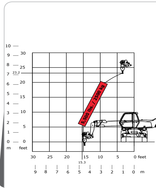
Rotation on Tires with 3 Ton Winch
