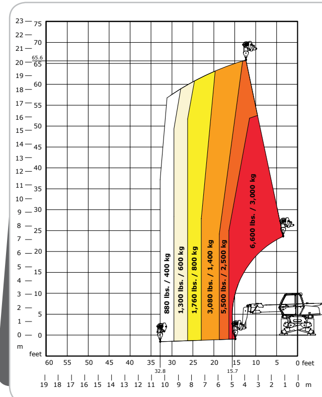
Rotation on Partial Stabilizers with 3 Ton Winch
