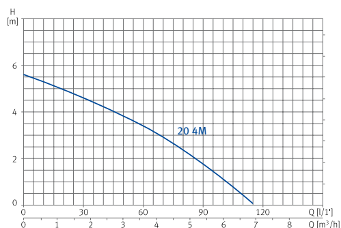
Jelleggörbe (2900 rpm)
