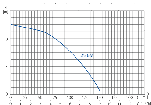
Jelleggörbe (2900 rpm)
