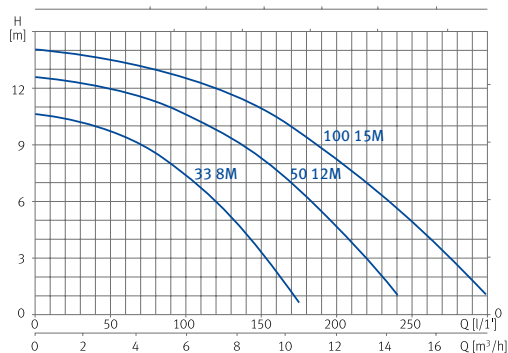
Jelleggörbe (2900 rpm)
