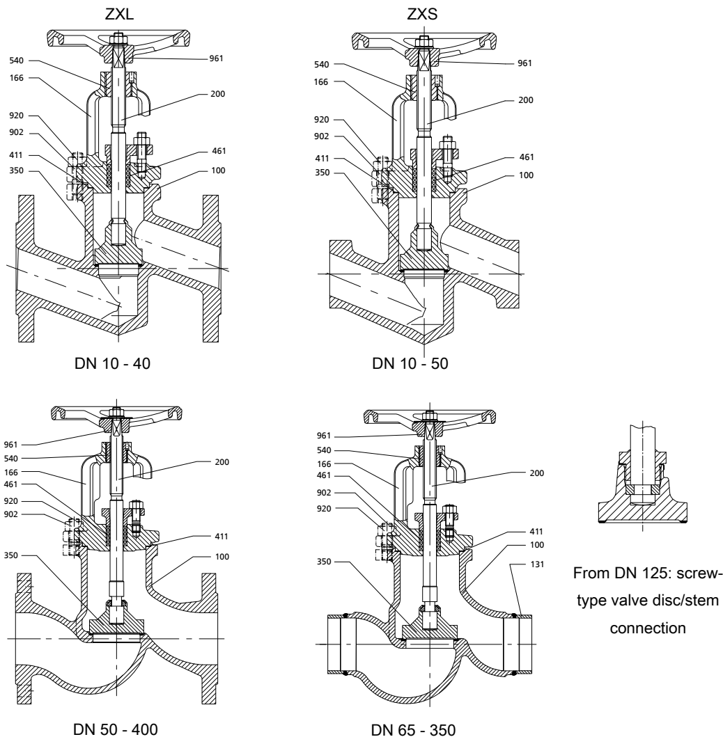
Fig. 1: Sectional drawings
