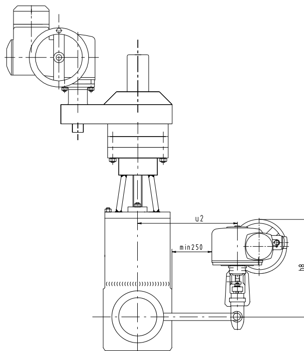
Model with spur gear and bypass with actuator
