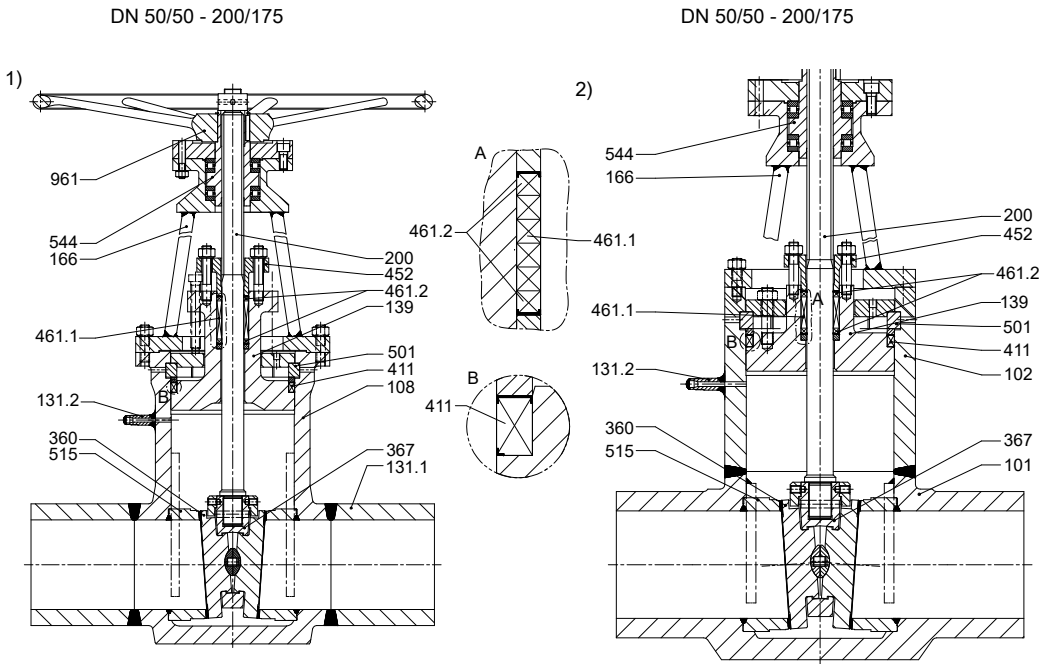
Fig. 1: Sectional drawings; ZTS 1) With connection branch extensions 2) Without connection branch extensions
