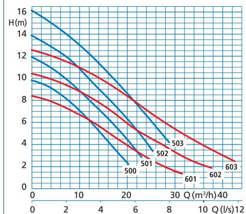
Jelleggörbék Ama-Porter 500/600
