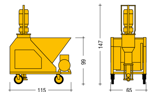
DIMENSIONS (cm)
