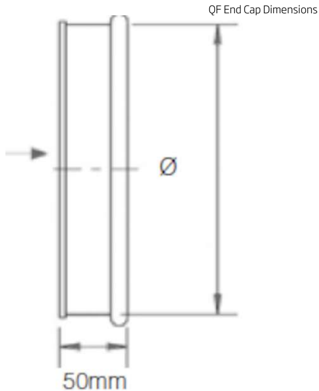
QF End Cap Dimensions, Z2012-XXX
