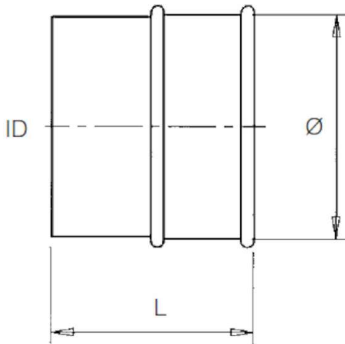
QF Ventilation adapter, Z2014-XXX
