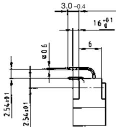
Solder pin angled
