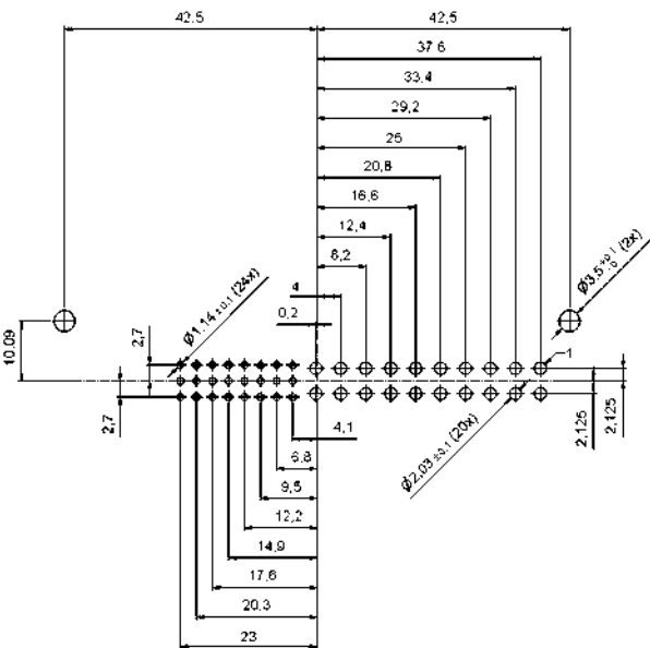
PCB-hole pattern
