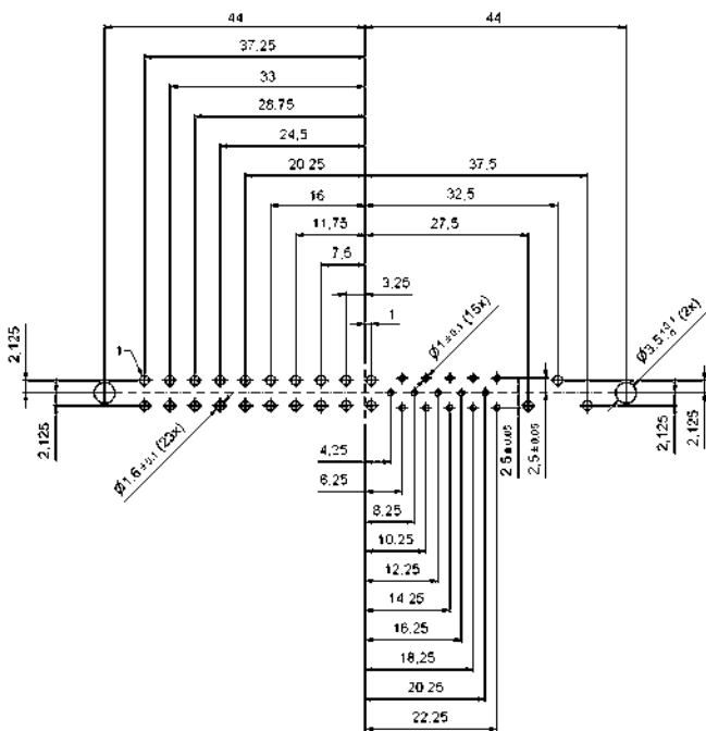
PCB-hole pattern
