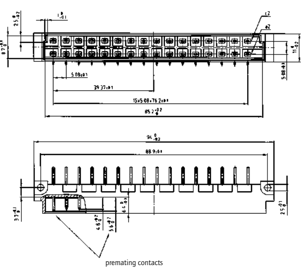
Solder pin angled
