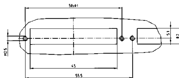
Panel cutout
