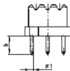
Solder pin straight
