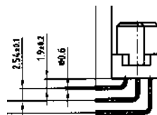
Solder pin angled
