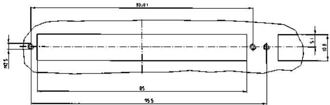
Panel cutout
