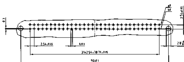
PCB-hole pattern
