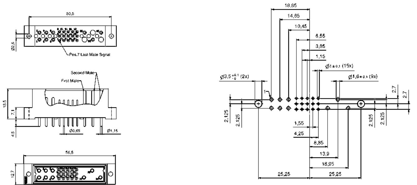
PCB-hole pattern
