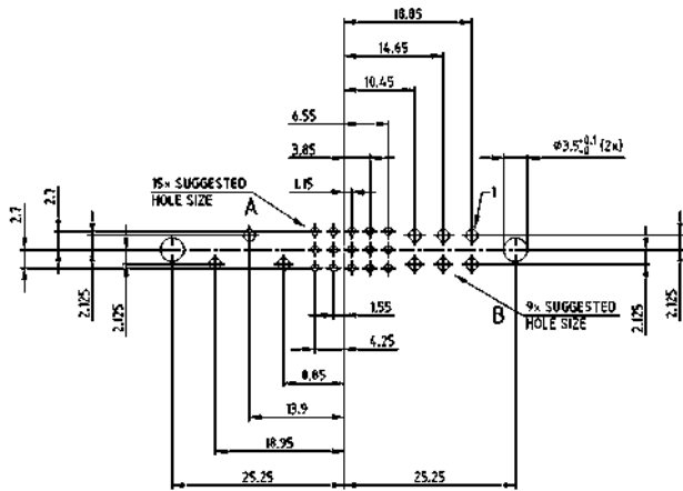
PCB-hole pattern
