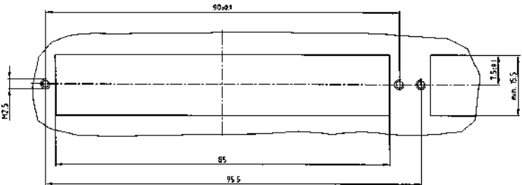
Panel cutout
