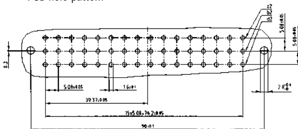
PCB-hole pattern
