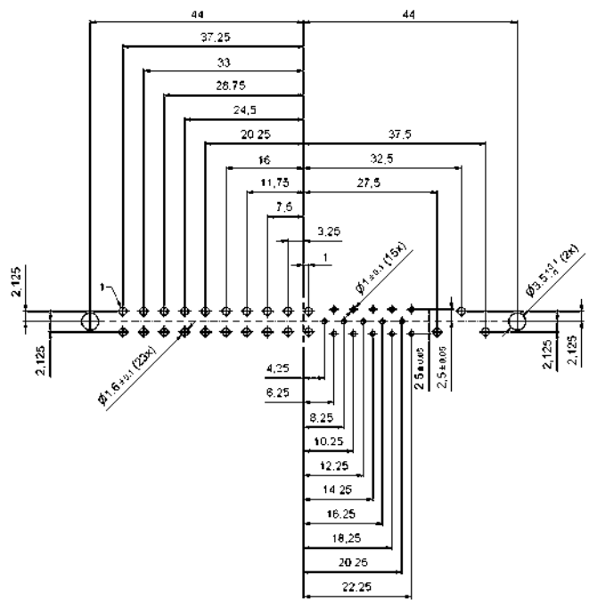
PCB-hole pattern
