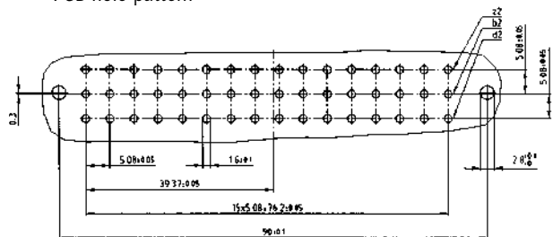
PCB-hole pattern
