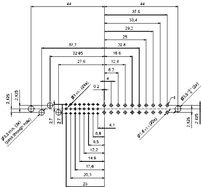
PCB-hole pattern
