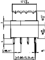
Solder pin straight
