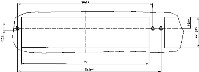
Solder pin straight
