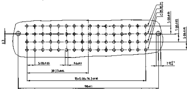
PCB-hole pattern
