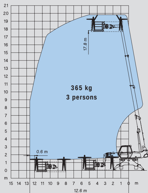
ROTATION ON STABILISERS WITH 365 KG PLATFORM ORH - 2,25/4 m
