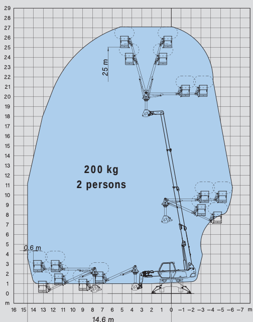
ROTATION ON STABILIZERS FULLY EXTENDED WITH AERIAL JIB 2 PLATFORM IN POSITIVE POSITION
