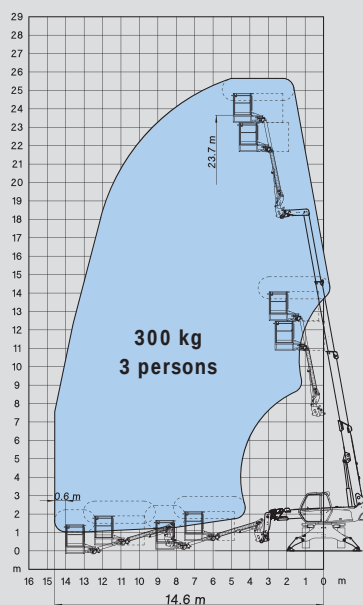
ROTATION ON STABILIZERS FULLY EXTENDED WITH AERIAL JIB 1
