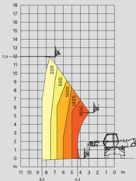
ROTATION ON WHEELS WITH FORKS
