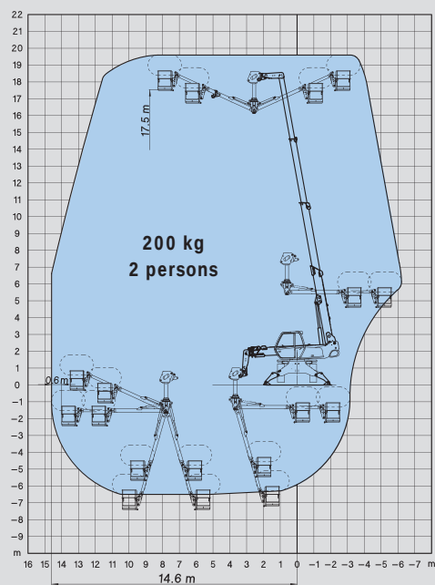
ROTATION ON STABILIZERS FULLY EXTENDED WITH AERIAL JIB 2 PLATFORM IN NEGATIVE POSITION
