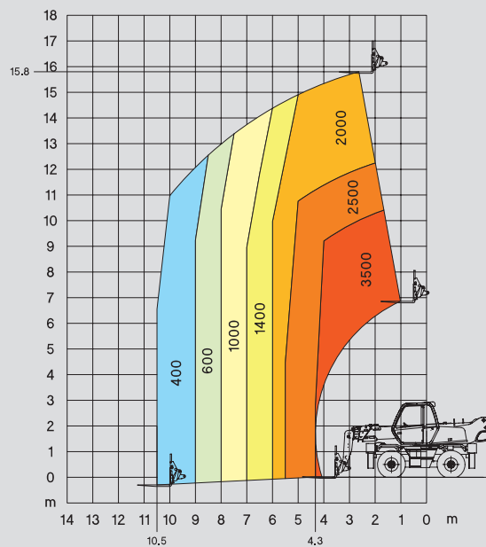
FRONTAL POSITION ON WHEELS WITH FORKS
