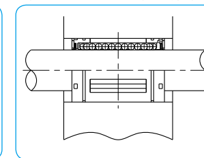
Figure D-7 Press Fit (TK type)
