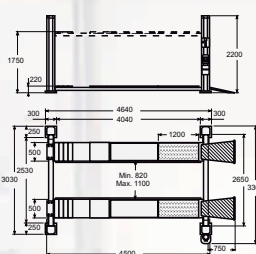
Art. 400/C - 401/C
