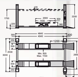
Art. 400/CSA - 401/CSA
