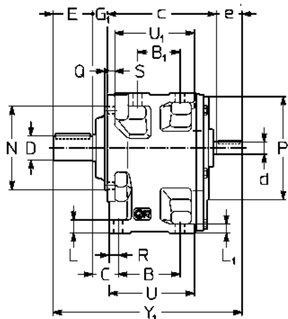
Standard design
