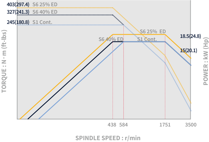
Main spindle_ Lynx 2600/M
