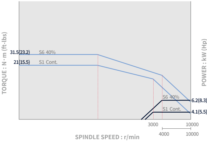
Rotary tool_ Lynx 2100M / LM / LMS OPTION
