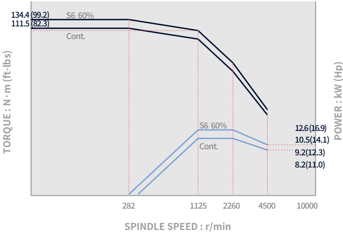
Main spindle_ Lynx 2100B / LB / MB / LMB / LMSB
