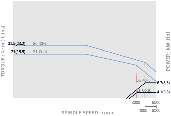
Rotary tool_ Lynx 2100M / LM / LMS
