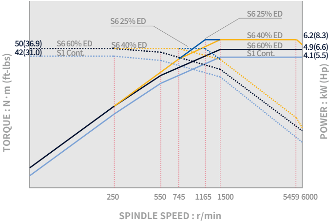
Rotary tool_ Lynx 2600M
