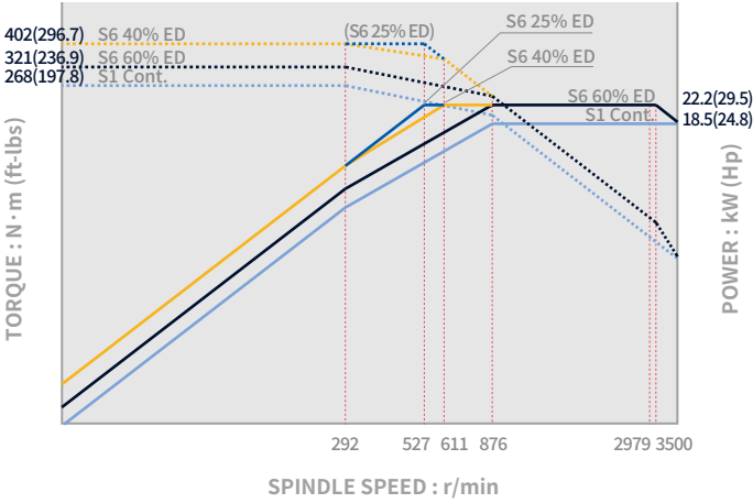
Main spindle_ Lynx 2600/M
